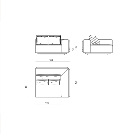
BOYY51 L 138 x H 62 x W 120 cm
