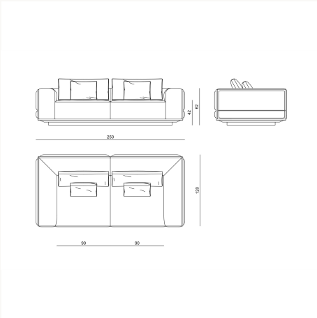
BOYY48 L 250 x H 62 x W 120 cm
