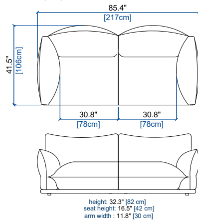
CANAPE 3 PLACES 3-SEAT SOFA SOFA 3 PLAZAS
