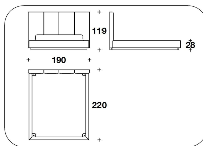
UR2 (LE1) LETTO PER MATERASSO / BED FOR MATTRESS 165x200 - 190x220x119H. - H.B.28cm 65x78 2/3 - 74 2/3x86 2/3x47H. - H.B.11"
