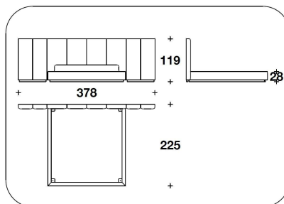
UR2 (KUSA) KING USA : LETTO PER MATERASSO / BED FOR MATTRESS 195x205 - 220x225x119H. - H.B.28cm 76 2/3x80 2/3 - 86 2/3x88 2/3x47H. - H.B.11"
