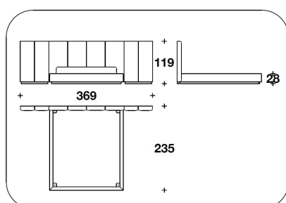
UR2 (CUSA) CALIFORNIA USA : LETTO PER MATERASSO / BED FOR MATTRESS 183x215 - 210x235x119H. - H.B.28cm 72x84 2/3 - 82 2/3x92 2/3x47H. - H.B.11"
