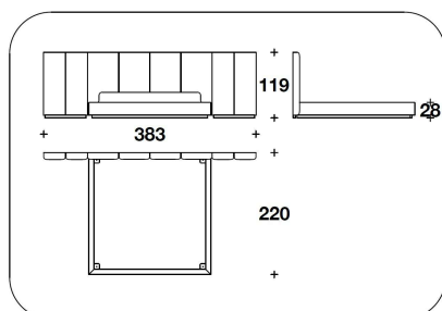
UR2 (LE7) LETTO PER MATERASSO / BED FOR MATTRESS 200x200 - 225x220x119H. - H.B.28cm 78 2/3x78 2/3 - 88 2/3x86 2/3x47H. - H.B.11"
