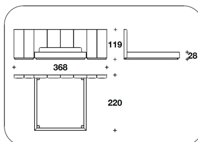
UR2 (LE2) LETTO PER MATERASSO / BED FOR MATTRESS 185x200 - 210x220x119H. - H.B.28cm 73x78 2/3 - 82 2/3x86 2/3x47H. - H.B.11"
