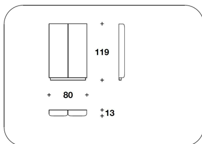
UR2 (SPODX) - UR2 (SPOX) SPONDA LATERALE / HEADBOARD SIDE 80x13x119H.cm 31 1/3x5x47H."
