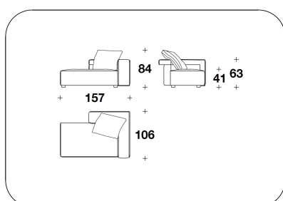
1BO (PEND) - 1BO (PENS) PENISOLA DX O SX / RIGHT OR LEFT PENINSULA 157x106x84H. - H.S.41cm 61 2/3x41 2/3x33H. - H.S.16 1/4"
