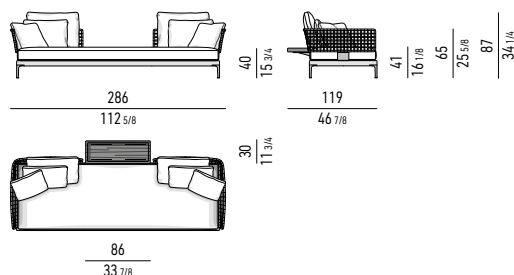
DIVANO OPEN CON TOP CM 286X119 OPEN SOFA WITH TOP CM 286X119
