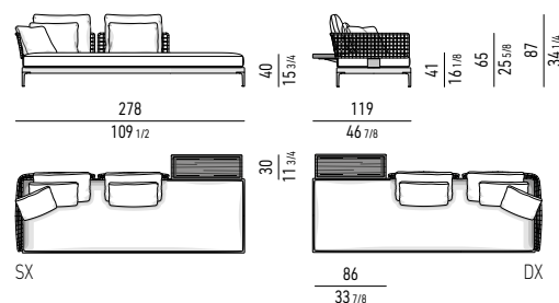
ELEMENTO TERMINALE PENISOLA CON TOP CM 278X119 OPEN-END ELEMENT WITH 1 ARMREST WITH TOP CM 278X119
