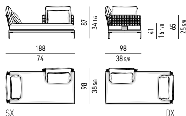
ELEMENTO TERMINALE DAYBED CM 188X98 DAYBED ELEMENT WITH 1 ARMREST CM 188X98
