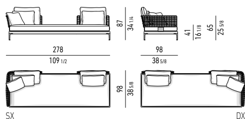
ELEMENTO TERMINALE OPEN CM 278X98 OPEN ELEMENT WITH 1 ARMREST CM 278X98
